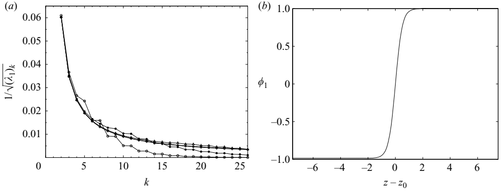
FIGURE 6. Solution of the eigenvalue problem (3.4) for the top pycnocline, with \rho_1=1.02 , \rho_2=1.05 , h_1=1 , obtained using a finite difference approximation on a uniform mesh of N points. (a) The 25 largest values of 1/\sqrt{(\lambda_1)_k} for the non-zero eigenvalues (\lambda_1)_k , k=2, \dots, 26 , with N=50 ( \circ ), 100 ( \bullet ), 200 ( \triangle ), 400 ( \blacktriangle ), 800 ( \diamond ). (b) Eigenfunction \phi_1 corresponding to (\lambda_1)_2 . The pycnocline is centred at z=z_0 .
