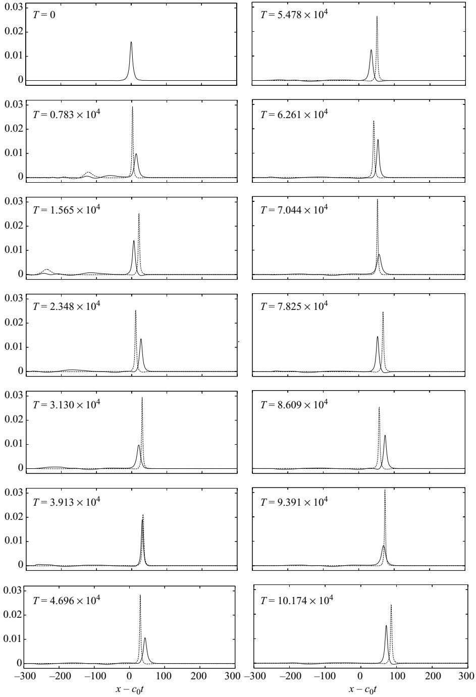
FIGURE 8. Upper and lower pycnocline amplitudes A(\xi, T) (solid) and B(\xi, T) (dashed) as a function of \xi = x - c_0 t at equal time intervals in the range 0 \leq T \leq 10.174 \times 10^4 , as indicated, where \rho_1 = 1.02 , \rho_2 = 1.11 , \rho_3 = 1.19 and h_2 = h_1 = 1 .
