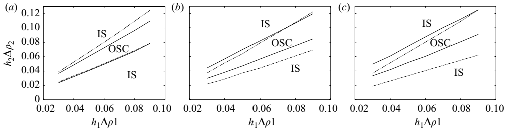
FIGURE 23. Regions in the parameter space h_1\Delta\rho_1 – h_2\Delta\rho_2 for which the chosen initial conditions lead to oscillations, as computed numerically (region between solid lines) and as follows from the asymptotic results (region between dashed lines). In all cases, h_1 = 1 , \rho_1 = 1.02 . (a) h_2 = 1.0 , (b) h_2 = 1.4 , (c) h_2 = 1.8 . The labels IS and OSC denote immediate separation and oscillations, respectively.
