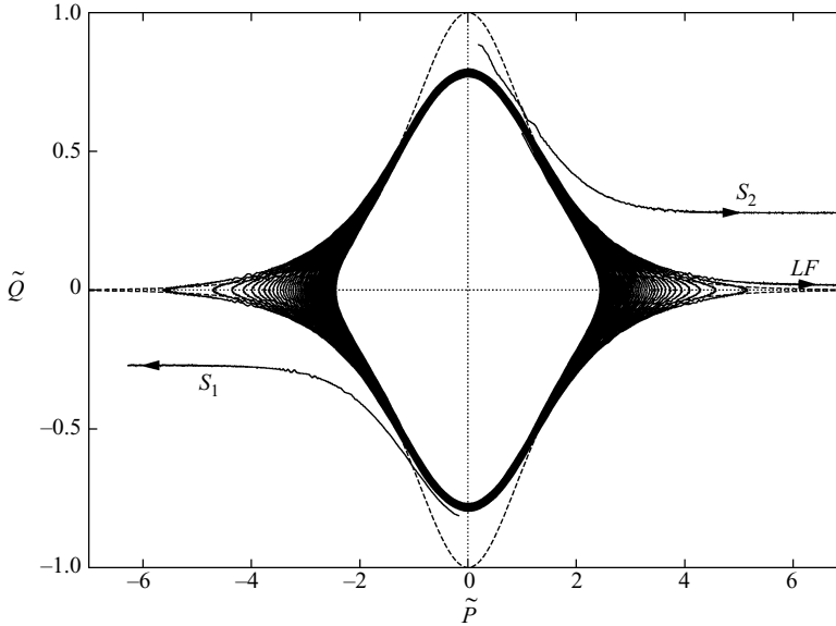
FIGURE 22. Phase plane for the numerical results; the orbit LF is a leapfrogging case, and the orbits S1 , S2 are those with immediate separation. The dashed curve is the separatrix for the model, equal to the dashed curve in figure 20.
