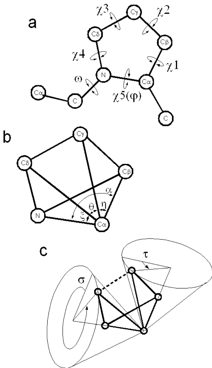
Figure 1. Schematic of the proline ring. (a) The torsions in the proline ring. \chi_5 and \varphi measure different torsions around the same central axis. (b) The tetrahedral angle in the proline ring has the apex at the C^\alpha atom and the N , C^\beta , C^\gamma and C^\delta atoms define the faces of the tetrahedral angle. The apical angles \alpha , \eta , \xi and \theta are also shown. (c) After fixing \alpha , \eta and \xi , the degrees of freedom consists of the \sigma and \tau dihedral angles racing out two cones. Fixing \theta will couple the values of \sigma and \tau .
