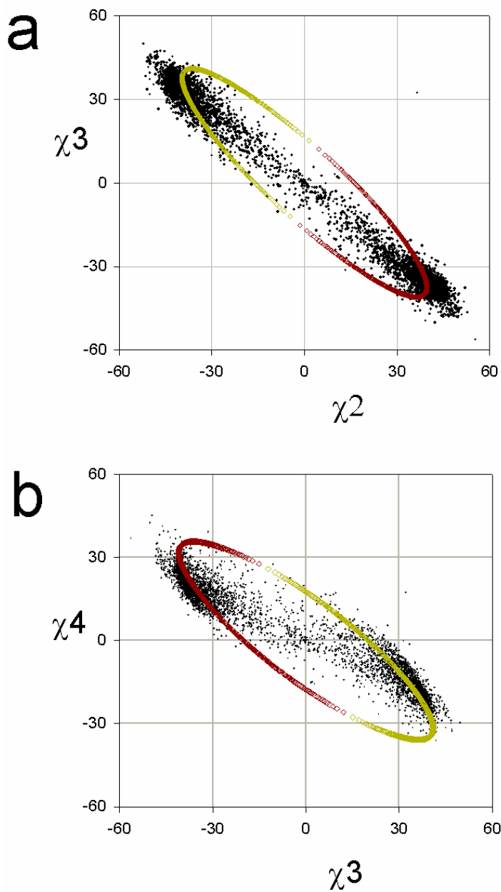
Figure 3. Correlations in the \chi torsions. (a) \chi_3 vs. \chi_2 and (b) \chi_4 vs. \chi_3 . The model curve passes through the two lobes of high density, where it is clear that the slope of the two lobes are determined by the model curve and is different to the curve formed by the sparse density of points in between. The colors of the curve represent the UP pucker (red) and the DOWN pucker (yellow).
