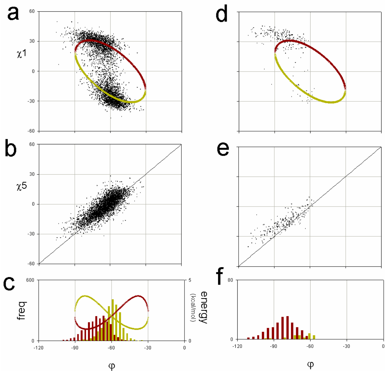
Figure 2. Distributions involving the \phi torsion. For the trans -Pro isomer, (a) Plot of \chi_1 vs. \phi , the curves represent the model based on the flexible tetrahedral angle, (b) Plot of \chi_5 vs. \phi where the line corresponds to conformations where there is ideal trigonal planar bonding at N and ideal tetrahedral bonding at C^\alpha , (c) the distributions of \phi for the DOWN pucker (red) and the UP pucker (yellow). (d), (e) and (f) are the corresponding plots for the cis -Pro isomer. The colors of the curve represent the UP pucker (red) and the DOWN pucker (yellow). The energy curve in (c) is due to the CHARMM C^\gamma - C^\delta -N angle term.
