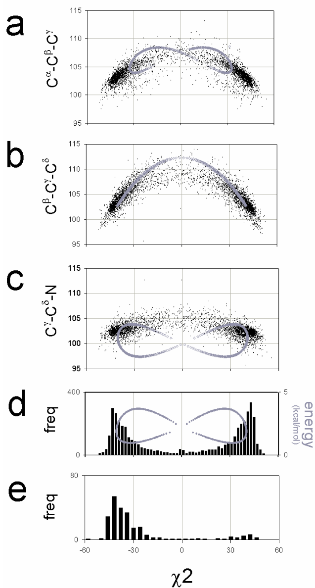
Figure 4. Bond angle strain in the proline ring as a function of \chi^2 for (a) C^\alpha-C^\beta-C^\gamma , (b) C^\beta-C^\gamma-C^\delta (c) C^\gamma-C^\delta-N . In the disfavored region at \chi^2 \sim 0^\circ , the model values of C^\gamma-C^\delta-N are found significantly below the observed values. This is the key strain that separates the puckers. \chi^2 frequency distributions for (d) the trans -Pro isomer (e) the cis -Pro isomer. The energy curve in (d) is due to the CHARMM C^\gamma-C^\delta-N angle term.
