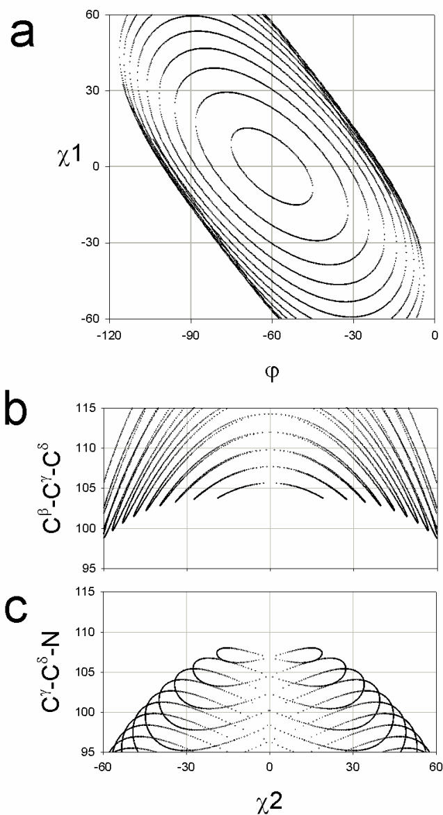
Figure 5. Family of curves for different values of C^\alpha-C^\beta-C^\gamma in (a) plot of \chi_1 vs. \phi , (b) C^\beta-C^\gamma-C^\delta vs. \chi_2 and (c) C^\gamma-C^\delta-N vs. \chi_2 . The parameterization of each curve is set for C^\alpha-C^\beta-C^\gamma in the range 50^\circ < C^\alpha-C^\beta-C^\gamma < 110^\circ in (a) 5^\circ steps; and in (b) & (c) 2^\circ steps. The curves with large cycles correspond to small C^\alpha-C^\beta-C^\gamma angles, whilst the curves with small cycles correspond to large C^\alpha-C^\beta-C^\gamma angles. As C^\alpha-C^\beta-C^\gamma approaches 111^\circ , the curves in (a) collapse to the point \chi_1 = 0^\circ , \phi = -60^\circ , in (b) to \chi_2 = 0^\circ , C^\beta-C^\gamma-C^\delta \sim 104^\circ , and in (c) to \chi_2 = 0^\circ , C^\gamma-C^\delta-N \sim 109^\circ and At this limit, the proline ring is planar.
