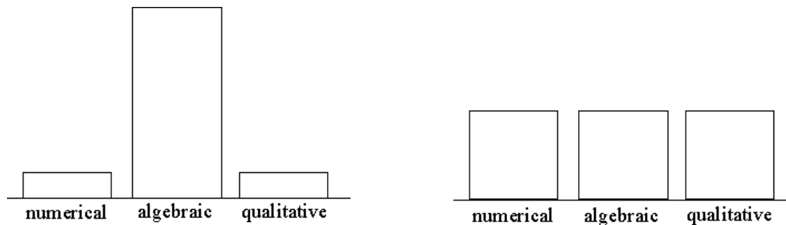
Figure 5: Approaches to the solution of a differential equation
