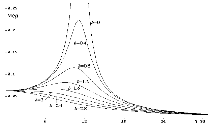
Figure 1: Resonance curves
