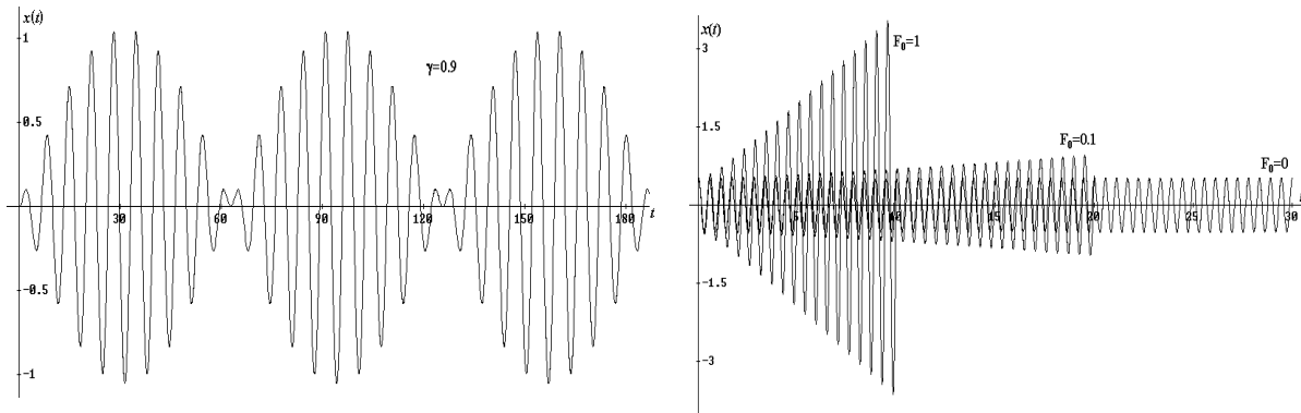
Figure 3: Beating and resonance
