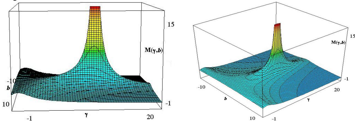
Figure 2: Three-dimensional representation of the resonance curves
