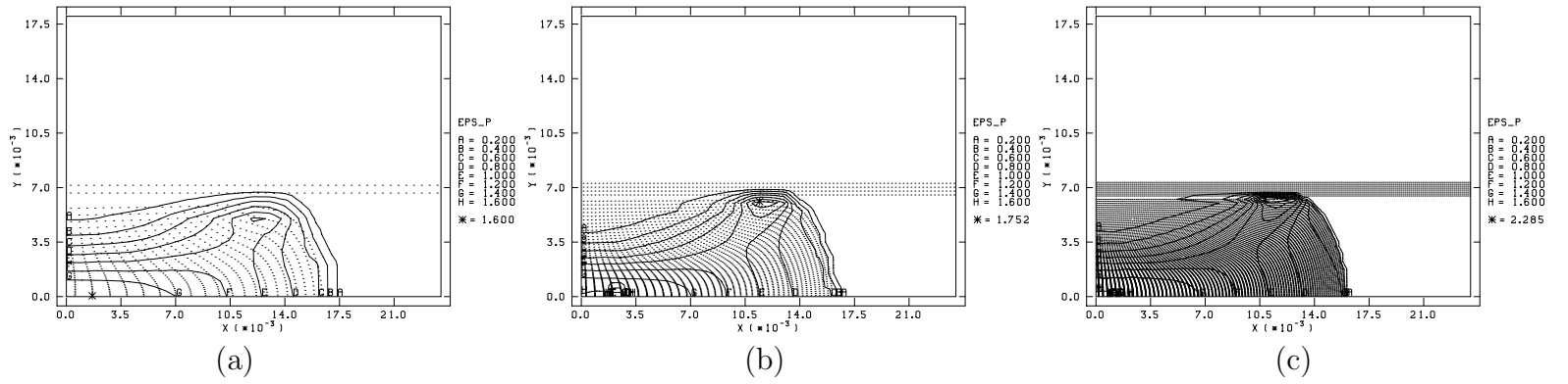
Figure 11: Contour plots of equivalent plastic strain using a timestep of 10^{-4} secs, which is 1000 times the explicit timestep, with a square spatial mesh size of (a) 1 mm (b) 0.5 mm and (c) 0.25 mm, on a side.
