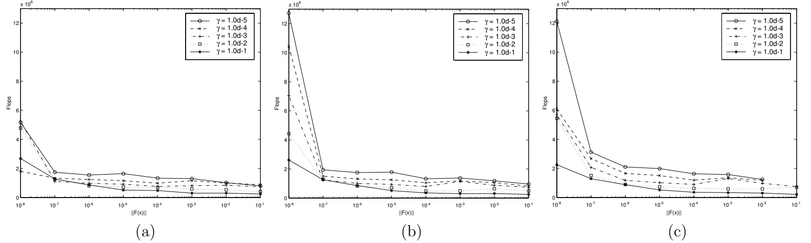
Figure 8: Effect of the linear parameter \gamma on the operations count for (a) h = 10^{-3} , (b) h = 10^{-4} , and (c) h = 10^{-5} and a time step 100 times that of the explicit case.
