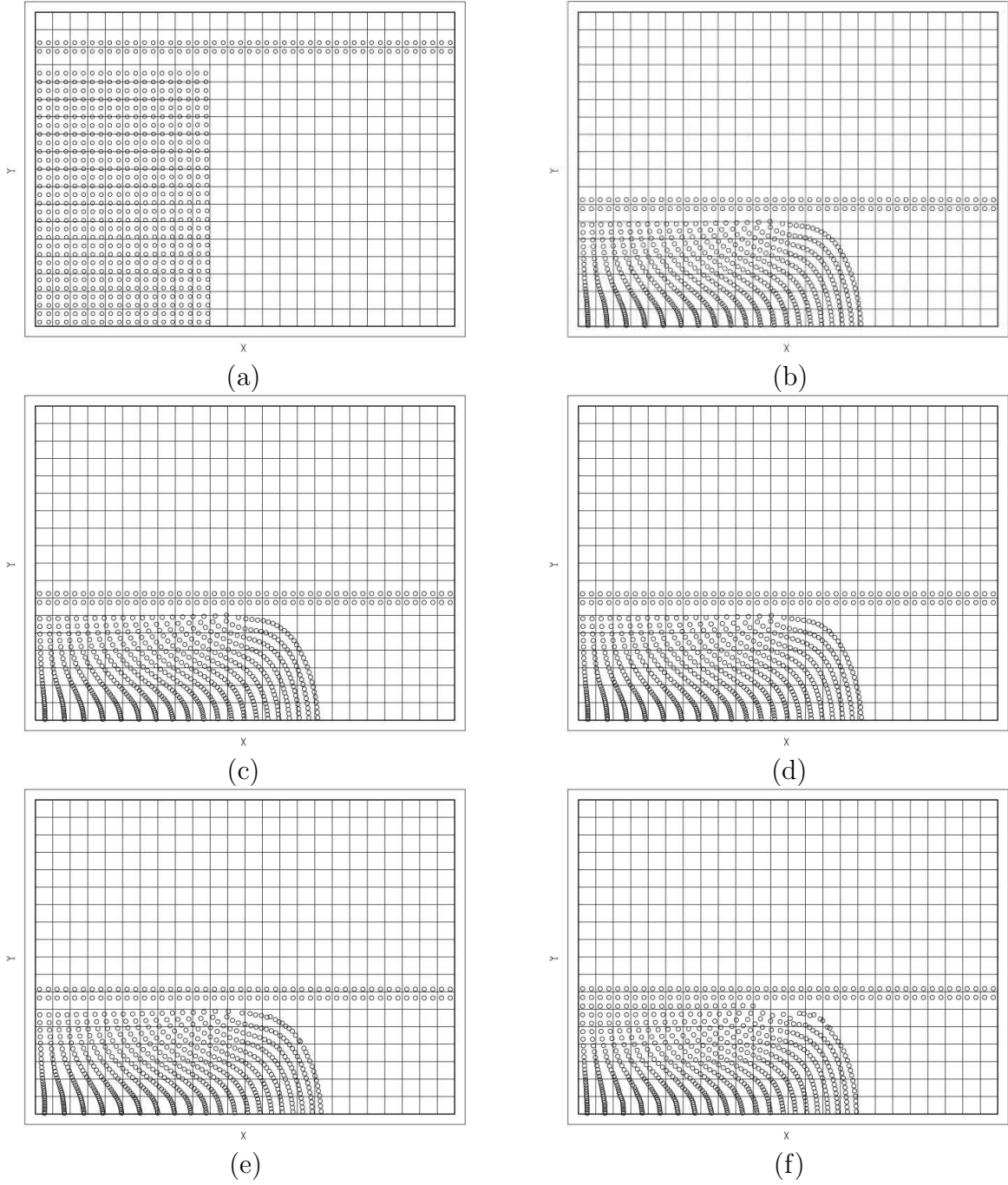
Figure 10: The upsetting problem. The initial configuration is shown in (a) and results after 60% upsetting in (b)-(f) for implicit cases with increasing time step size.
