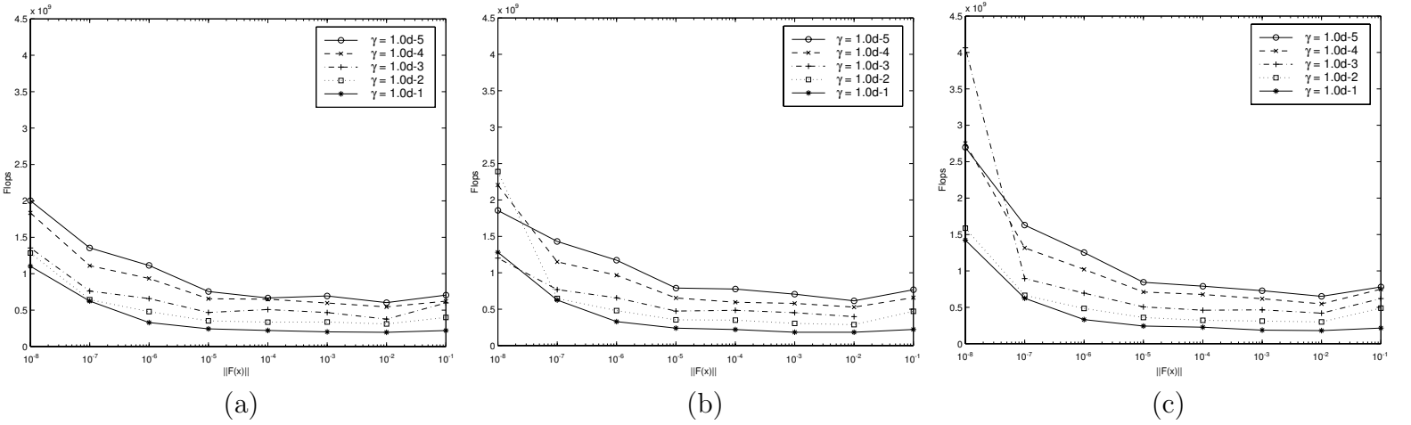
Figure 7: Effect of the linear parameter \gamma on the operations count for (a) h = 10^{-3} , (b) h = 10^{-4} , and (c) h = 10^{-5} and a time step ten times that of the explicit case.
