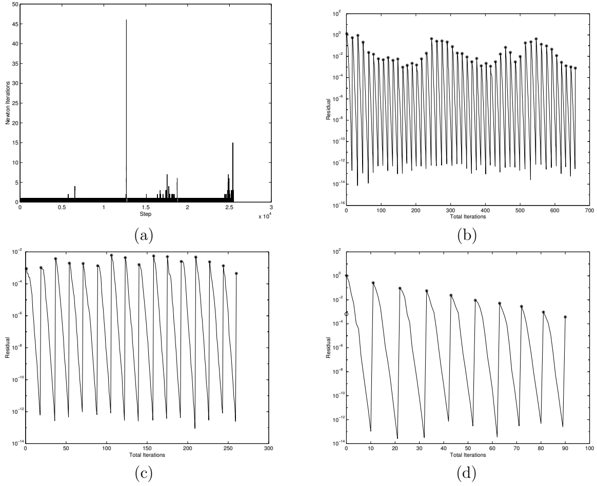
Figure 9: Effect of line search on nonlinear residuals. The number of nonlinear iterations as a function of time step is shown in (a), nonlinear and linear residuals for steps 12694 and 25402 without a line search are shown in (b) and (c), respectively, and with a line search in (d).
