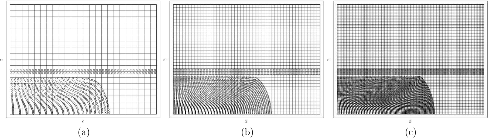
Figure 13: The upsetting problem. The results after 60% upsetting in (a)-(c) for implicit cases with increasingly refined spatial meshes. The timestep is kept fixed at 10^{-4} secs, which is 1000 times the explicit timestep for the coarse mesh.
