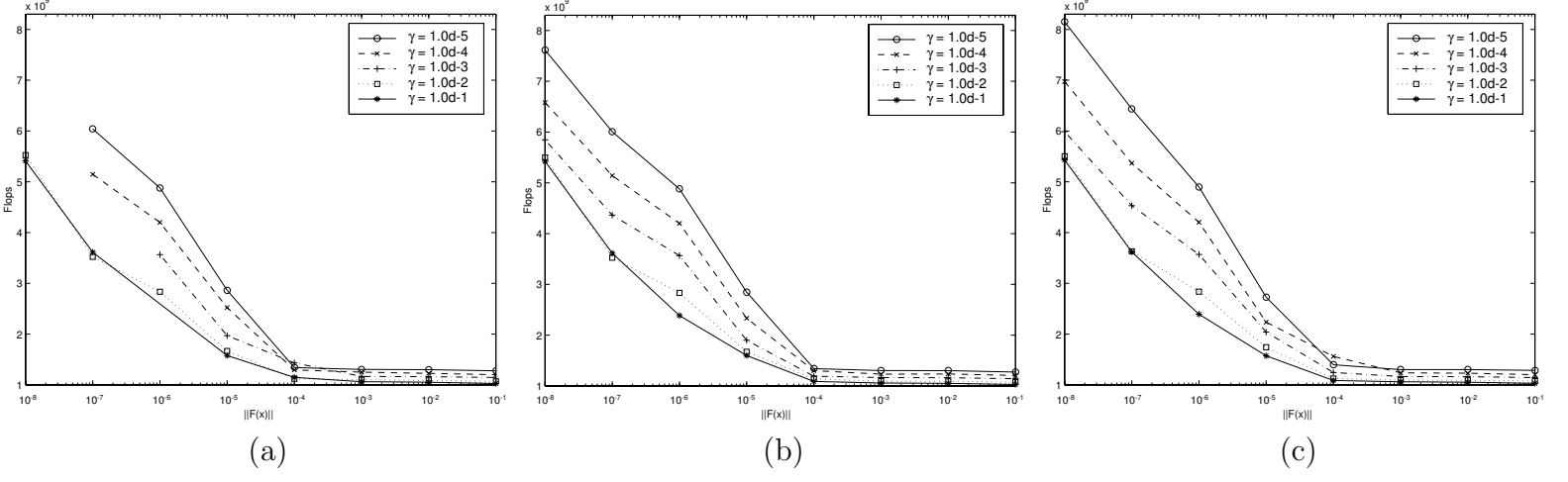
Figure 6: Effect of the linear parameter \gamma on the operations count for (a) h = 10^{-3} , (b) h = 10^{-4} , and (c) h = 10^{-5} and a time step equal to the explicit case.
