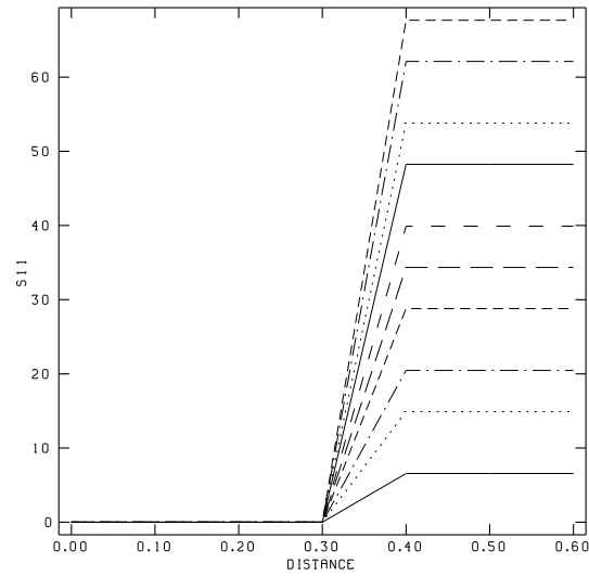
Figure 4: The elastic-plastic bar under tension. Stress in the middle of the bar as a function of distance along the bar at various times.
