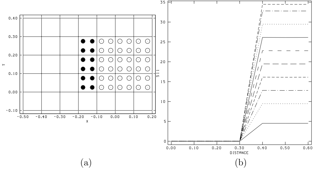
Figure 1: The bar under tension. Initial configuration of the bar is shown in (a), stress in the middle of the bar as a function of distance along the bar for the implicit case is shown in (b) for 10 different times.
