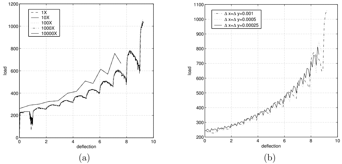
Figure 12: Load on the rigid platen (kN) as a function of deflection (mm). In (a) the spatial mesh is kept fixed and the timestep is varied and in (b) the timestep is fixed at 10^{-4} secs, which is 1000 times the explicit step size on the coarse mesh, and the spatial mesh is refined.
