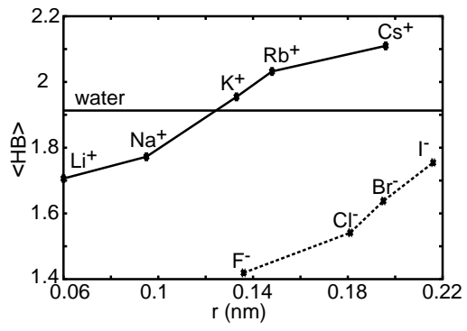
Figure 4: The average number of the water-water hydrogen bonds, \langle HB \rangle , per water molecule in the first shell around various ions at T^*=0.20 .
