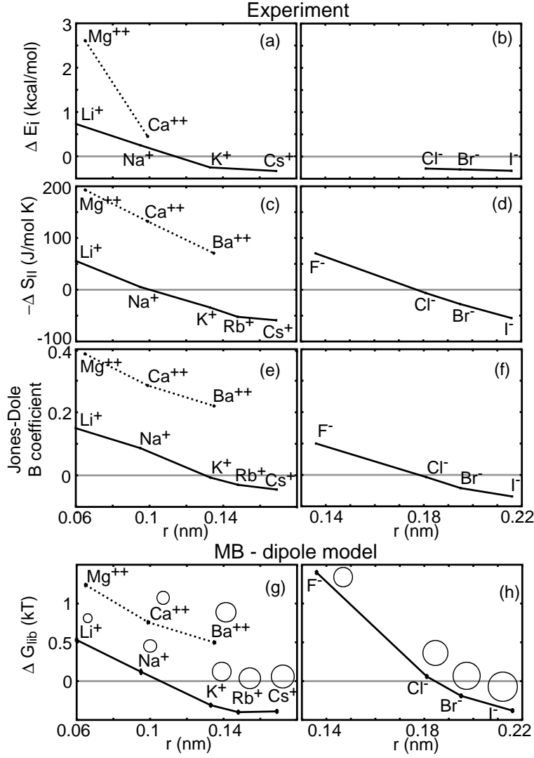
Figure 6: The MB-dipole model reproduces the dependence on ion radius of chaotropic and kosmotropic properties. The activation energy of Samoilov, \Delta E_i ([15]), changes in entropy, -\Delta S_{II} ([17]), and Jones-Dole B coefficients ([18]) all at 298K, are compared to the MB-dipole model liberation free energy, \Delta G_{lib} , at T^*=0.20 . \sigma for Mg^{++} , Ca^{++} , and Ba^{++} were taken to be 0.26, 0.39, and 0.53 l_{HB} , scaled from ionic crystal radii [55]. Zero values indicate the transition between kosmotropes (greater than zero) and chaotropes (less than zero). Circles indicate relative ion radii.
