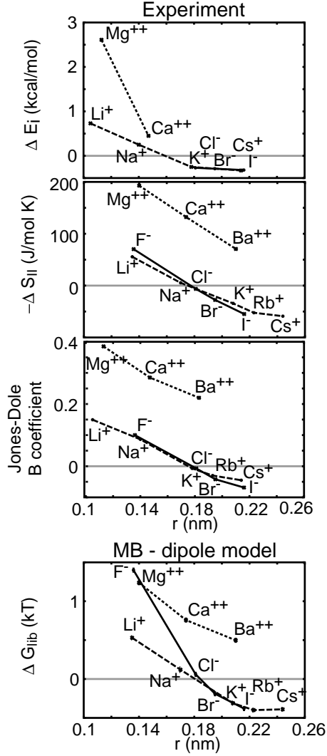
Figure 7: A universal curve showing that chaotropic and kosmotropic properties depend on electrostatic potential at the ion. The activation energy of Samoilov, \Delta E_i ([15]), changes in entropy, \Delta S_{II} ([17]), and Jones-Dole B coefficients ([18]) all at 298K, as compared to the MB-dipole model liberation free energy, \Delta G^{lib} , are shown for sets of cations and anions at T^*=0.20 . A single distance shift was chosen to overlay the cations onto the anions, indicating that the physical basis for this asymmetry is the asymmetry of the dipole in water.
