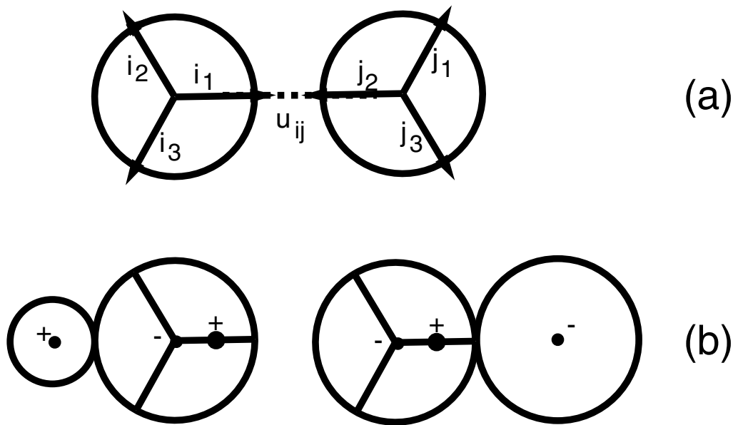
Figure 1: The MB-dipole model. (a) Two MB-dipole waters forming a hydrogen bond. (b) A cation and an MB-dipole water oriented in its most favorable orientation (180 degrees with respect to the vector connecting the molecular centers). Also an anion and a water oriented in its most favorable orientation (0 degrees).
