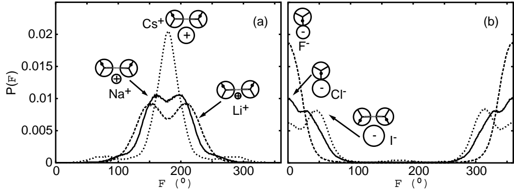
Figure 3: Angular distribution functions for waters in the first shell around an ion, for (a) cations and (b) anions at T^*=0.20 . Large cations help promote hydrogen bonding of neighboring waters, leading to a single peak. For small cations, the electrostatic mechanism competes with the hydrogen bond mechanism for ordering waters. The reverse applies to anions. For small anions, the electrostatic mechanism dominates; for large anions, electrostatic and hydrogen bonding mechanisms compete.
