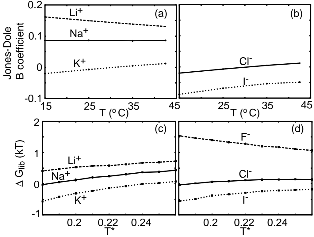
Figure 8: The MB-dipole model reproduces the temperature dependence of chaotrope and kosmotrope behavior. The temperature dependence of Jones-Dole viscosity coefficients, B(T) , from experiments ([18]) for (a) cations and (b) anions, and the temperature dependence of liberation free energy, \Delta G^{lib} , from the MB-dipole simulations for (c) cations and (d) anions are shown.
